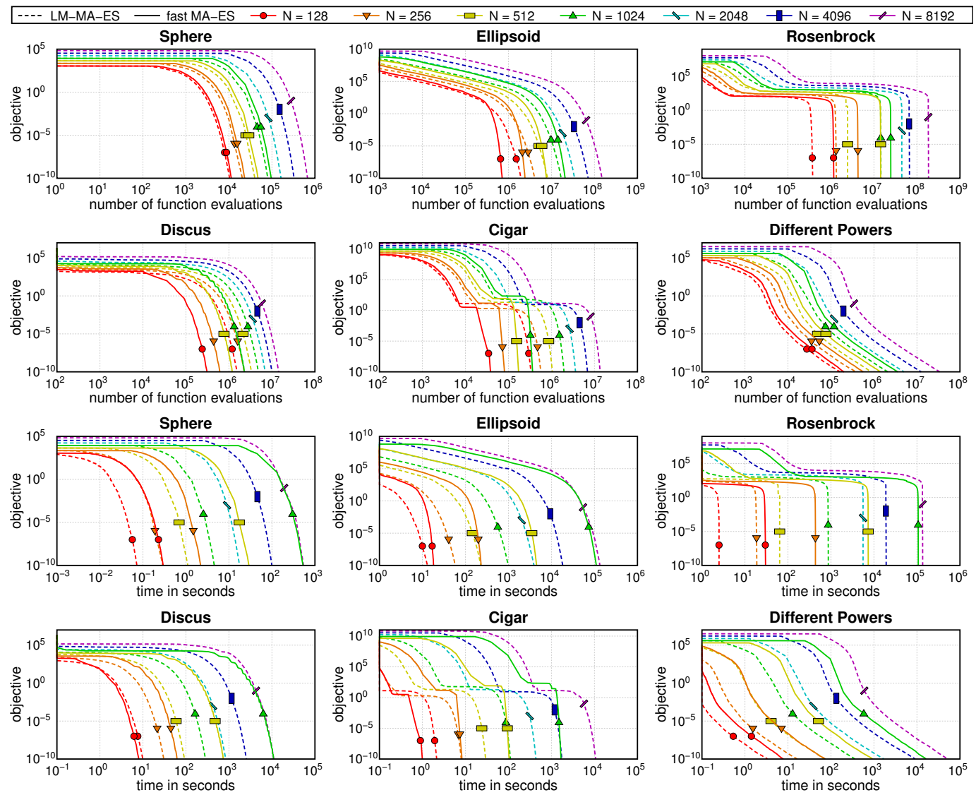
Fig. 2. Runtime in number of function evaluations (rows 1–2) and seconds (rows 3–4) of LM-MA-ES in 128 to 8192 dimensions and fast MA-ES in 128 to 1024 dimensions on six standard benchmark problems.
