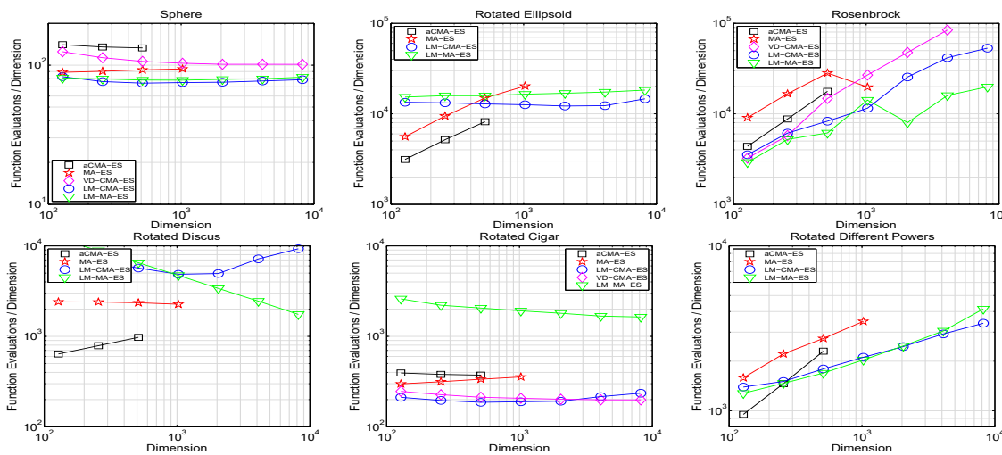
Fig. 3. Median number of function evaluations (out of 5 runs) required to achieve a target objective function value of f_{tar} = 10^{-10} . The results of VD-CMA-ES are shown only on functions where the algorithm succeeded achieving f_{tar} . Some results for CMA-ES and MA-ES are missing due to their extremely long runtimes (note that the vertical axis shows function evaluations, not runtime).
