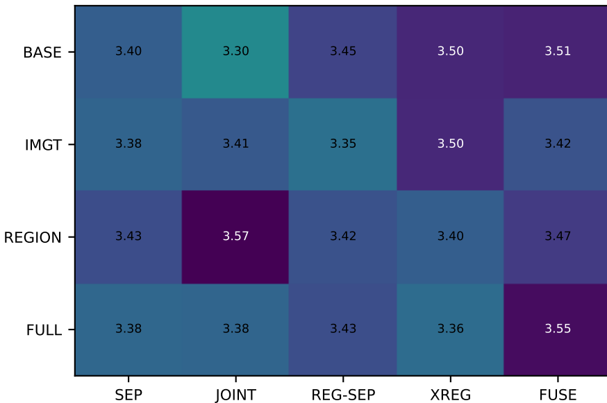
AbLang1
