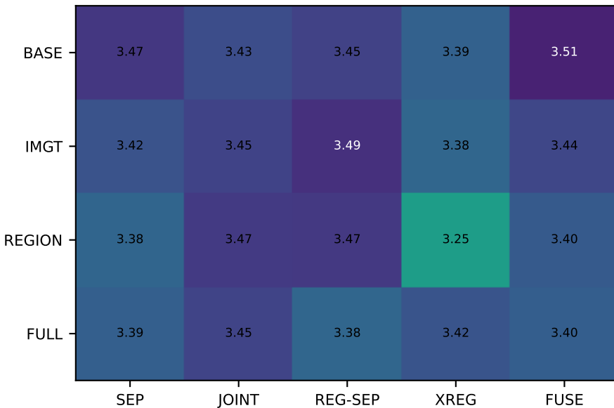
CurrAb (separate-chain)
