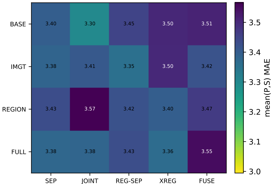
AbLang1: mean(P,S)
