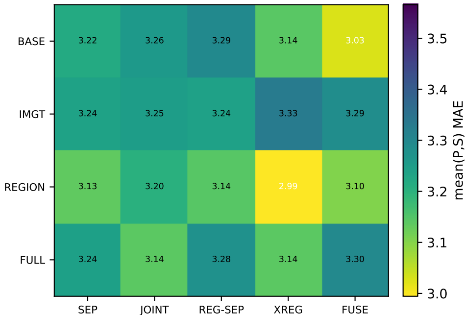
AbLang2 (separate-chain): mean(P,S)
