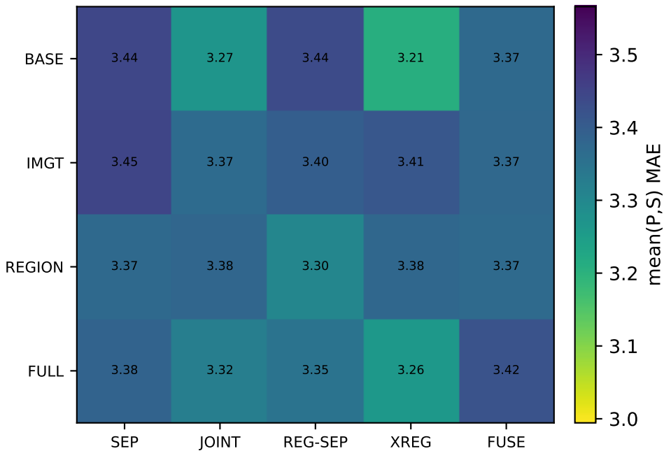
ESM-1b: mean(P,S)
