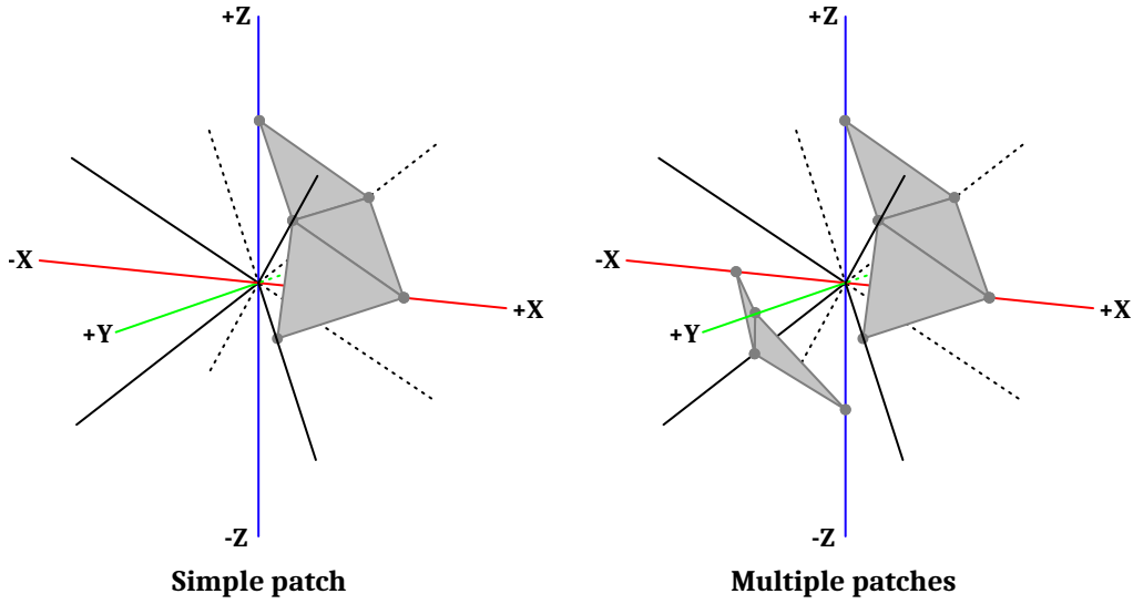
Figure 12: Two mergeable candidate topologies; note that the multiple patches example must have each patch/island merged individually.
