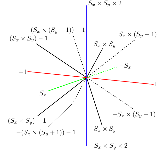
Figure 14: Visual depiction of the table of sample index offsets, for the body-centered tetrahedron arrangement, on even slices of the Z axis. S_x is defined to be the number of samples present in the array on the X axis, while S_y is defined likewise for the Y axis.
