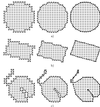
Figure 8: The elastic surface nets algorithm demonstrated in 2D. From left to right, each image shows a greater degree of relaxation (Gibson, 1998).
