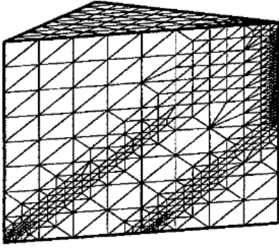
Figure 10: Illustration of inconsistent surface tessellation density (Bey, 1995).
