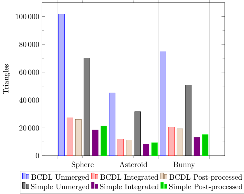
Figure 24: Triangle counts of output meshes from all test cases. The noticeable spikes are associated with a lack of merging applied.
