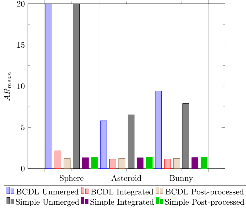
Figure 26: Mean aspect ratios - AR_{mean} - of triangles from output meshes from all test cases. Note that the 'BCDL Unmerged' and 'Simple Unmerged' results for the sphere mesh are much larger than all other results. See section 7 for numerical values.
