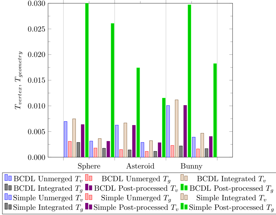
Figure 25: Vertex and geometry pass execution time from all test cases.
