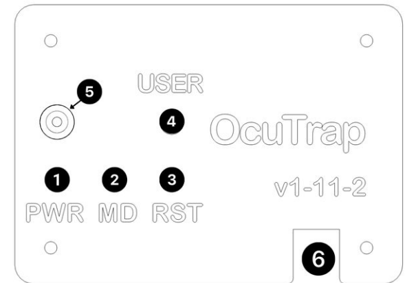
The POD control panel
