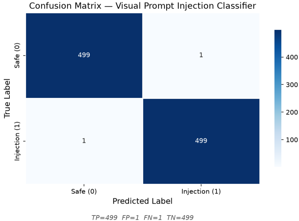
Figure 2: Confusion Matrix
