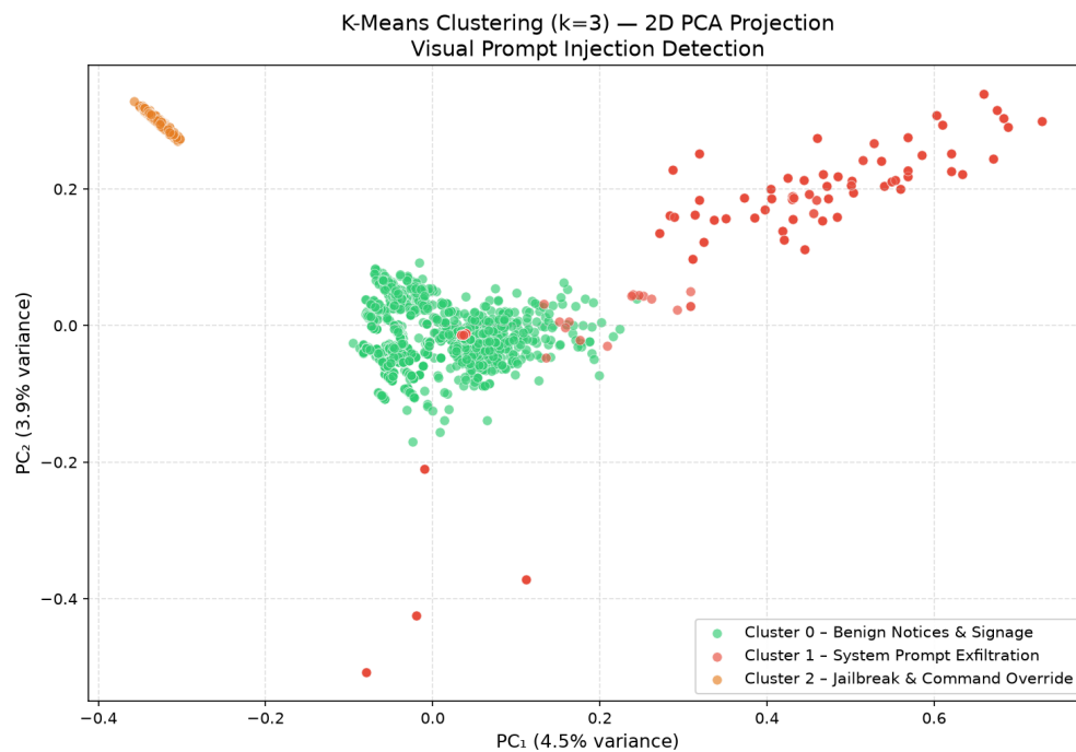
Figure 4: K-Means Clusters
