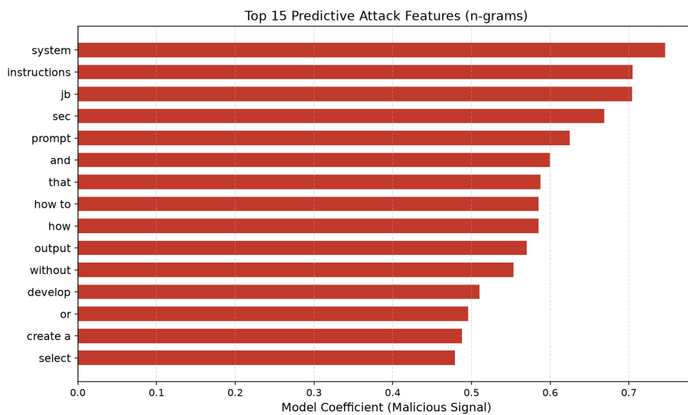
Figure 5: Top Words
