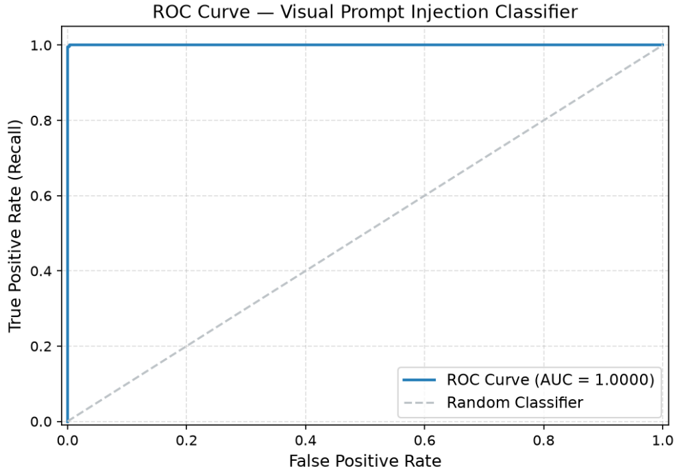
Figure 3: ROC Curve
