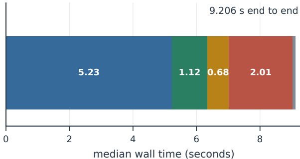
(a) Complete proof pipeline, H = 26
