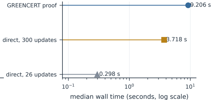
(b) Matched continuation controls
