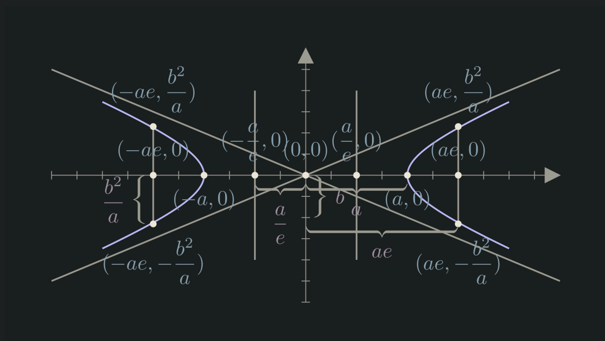
Figure 3: \frac{x^2}{a^2} - \frac{y^2}{b^2} = 1
