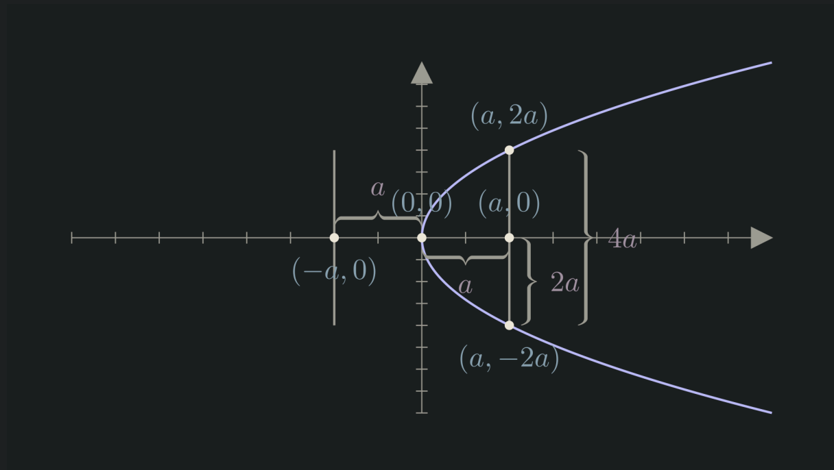
Figure 1: y^2 = 4ax
