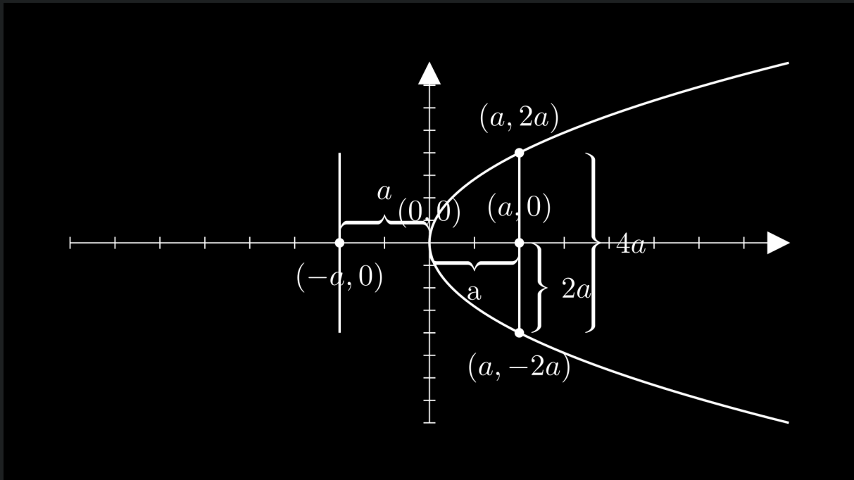
Figure 1: y^2 = 4ax
