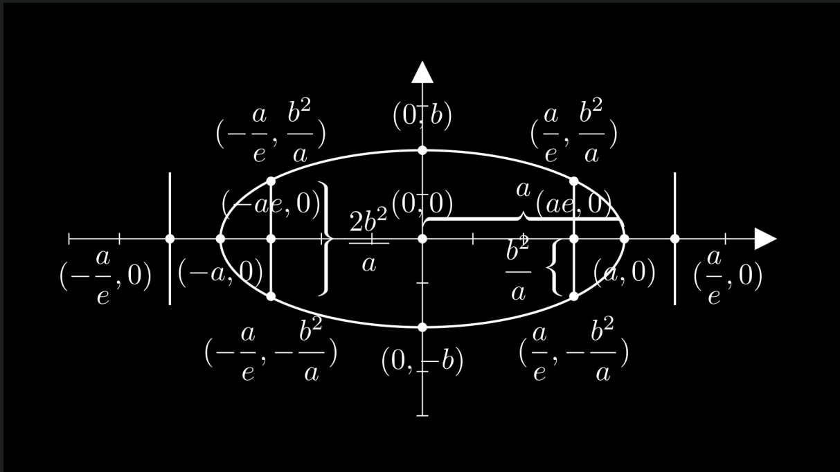
Figure 2: \frac{x^2}{a^2} + \frac{y^2}{b^2} = 1
