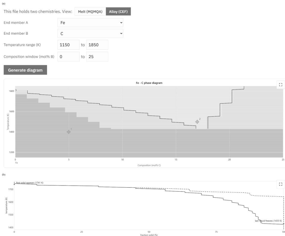
Figure 6: One unified (.utdb) file, two physics, calculated in the browser. (a) The steelmaking database loaded with the Melt/Alloy view toggle on Alloy; the engine calculates the Fe-C phase diagram through the magnetic compound energy formalism, rendered over a 0-25 mol% C composition window (the equilibrium always solves the whole join), with two tapped compositions pinned. (b) Scheil solidification for the same join at 4 mol% C, first solid at 1741 K and the residual liquid frozen by 1433 K, against the equilibrium lever-rule path (dashed). The file's slag half is a Modified Quasichemical Model liquid; no legacy container holds both models at once.
