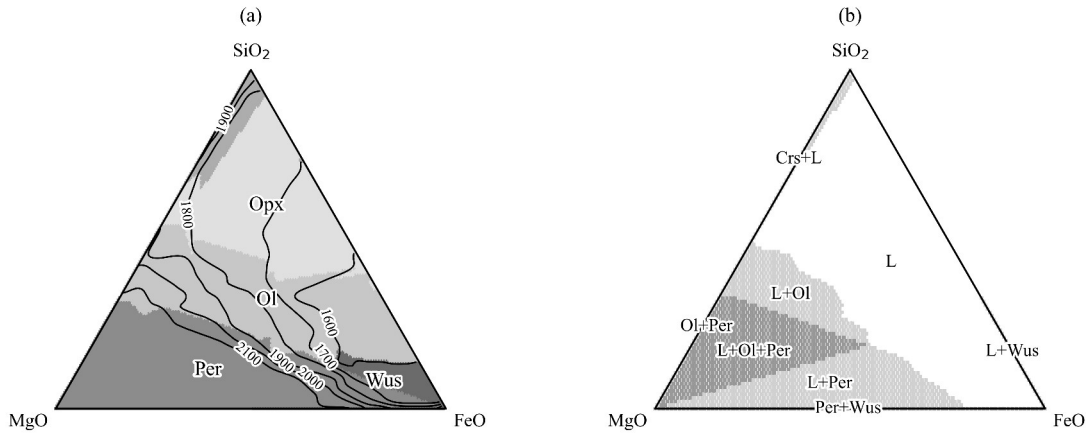
Figure 3: The assessed \text{FeO-MgO-SiO}_2 system calculated from the shipped database files. (a) Liquidus projection: primary crystallizing phase fields, with liquidus isotherms labeled in K. (b) Isothermal section at 1873 K: stable phase assemblages, shaded by the number of solid phases present. Phase labels: L liquid, Crs cristobalite, Ol olivine, Opx orthopyroxene, Per periclase, Wus wustite.
