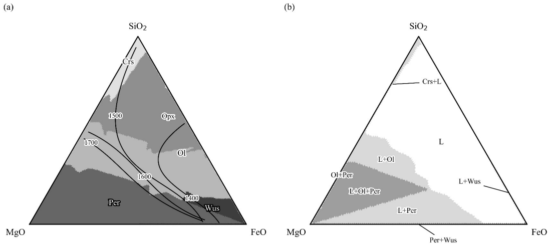
Figure 3: The assessed \text{FeO-MgO-SiO}_2 system calculated from the shipped database files. (a) Liquidus projection: primary crystallizing phase fields, with liquidus isotherms labeled in °C. (b) Isothermal section at 1600 °C: stable phase assemblages, shaded by the number of solid phases present. Phase labels: L liquid, Crs cristobalite, Ol olivine, Opx orthopyroxene, Per periclase, Wus wustite.
