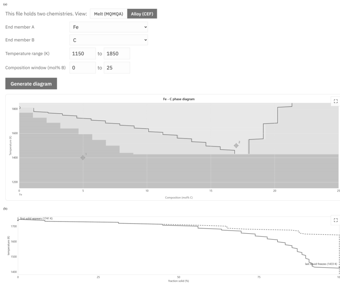
Figure 6: One unified (.utdb) file, two physics, calculated in the browser. (a) The steelmaking database loaded with the Melt/Alloy view toggle on Alloy; the engine calculates the Fe-C phase
