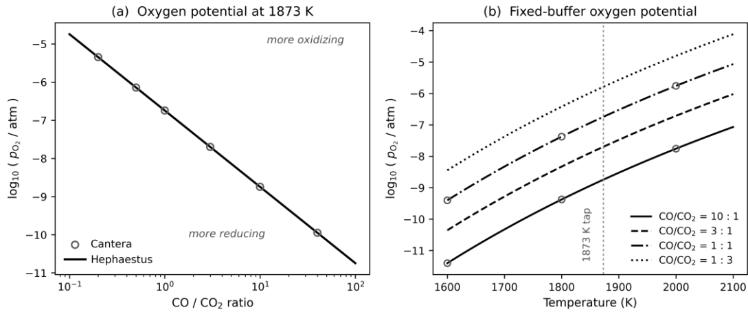
Figure 7: The gas calculator as a steelmaking worked example, the equilibrium of a carbon-oxygen furnace gas by the Hephaestus gas engine (the NASA-polynomial element-potential solver compiled into the browser), with Cantera as the independent check. (a) Oxygen partial pressure against the CO to CO 2 ratio at the 1873 K tap temperature: a lower ratio is more oxidizing and drives iron into the slag as FeO, a higher ratio is more reducing and decarburizes the steel. (b) The same oxygen potential against temperature for four fixed CO to CO 2 buffers, showing that a given gas grows more oxidizing as it heats; the dashed line marks the tap temperature. Open circles are Cantera, agreeing to about 10 -5 mole fraction across the field.
