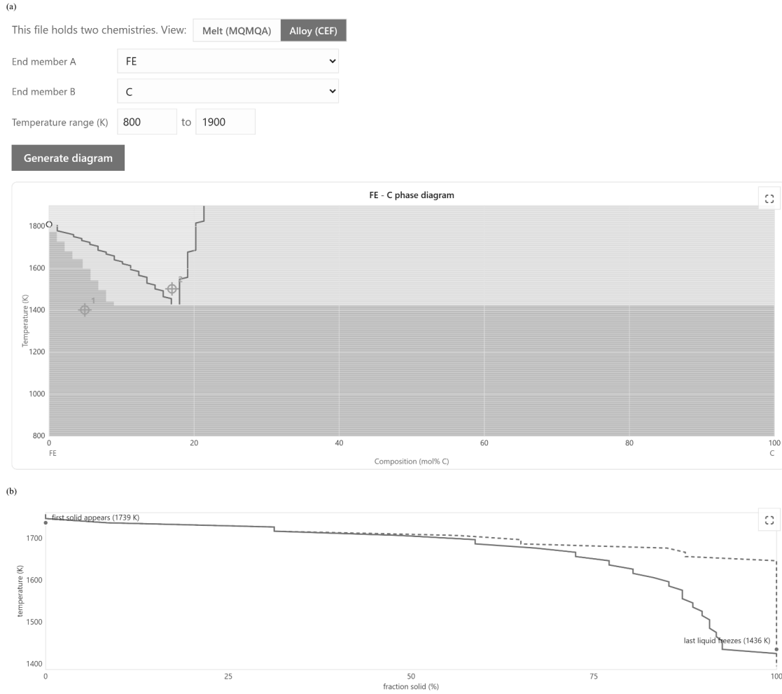
Figure 6: One unified (.utdb) file, two physics, calculated in the browser. (a) The steelmaking database loaded with the Melt/Alloy view toggle on Alloy; the engine calculates the Fe-C phase diagram through the magnetic compound energy formalism, with two tapped compositions pinned. (b) Scheil solidification for the same join at 4 mol% C, first solid at 1739 K and the residual liquid frozen by 1436 K, against the equilibrium lever-rule path (dashed). The file's slag half is a Modified Quasichemical Model liquid; no legacy container holds both models at once.
