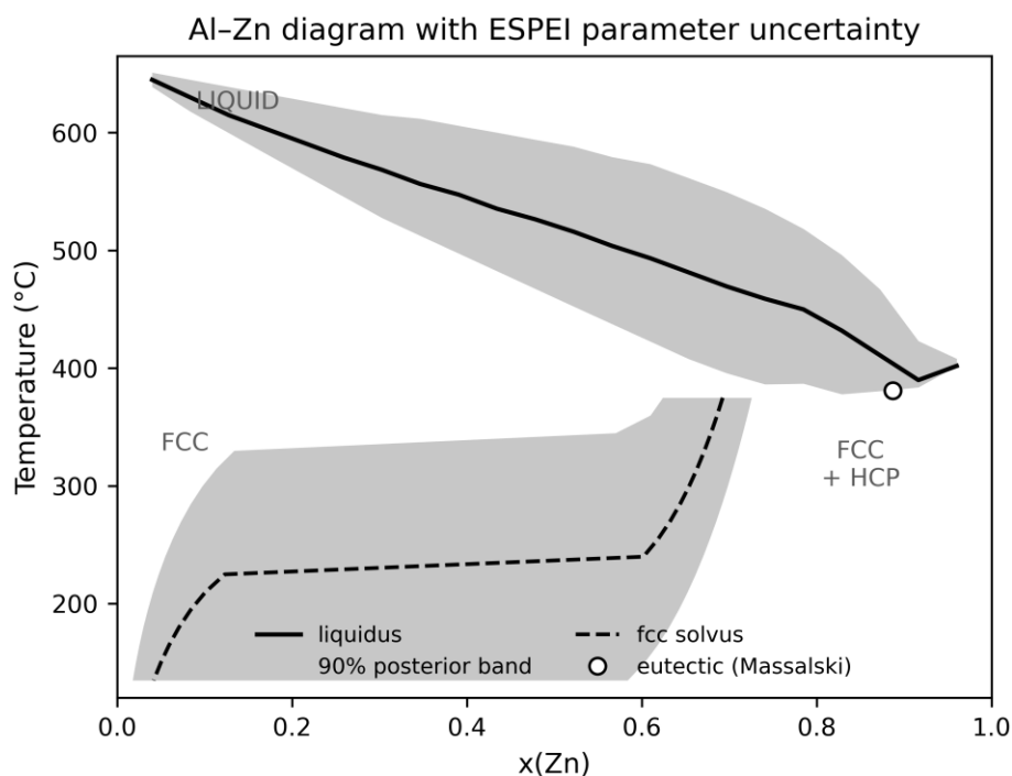
Figure 8: Al-Zn phase diagram with ESPEI parameter uncertainty. The liquid and face-centred-cubic (fcc) excess parameters were refit by Markov-chain Monte Carlo to the measured liquid enthalpy of mixing (Debski et al., digitised from Dinsdale et al. [44]) and the assessed phase
