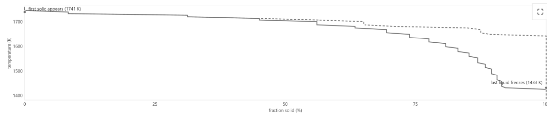
Figure 6: One unified (.utdb) file, two physics, calculated in the browser. (a) The steelmaking database loaded with the Melt/Alloy view toggle on Alloy; the engine calculates the Fe-C phase diagram through the magnetic compound energy formalism, rendered over a 0-25 mol% C composition window (the equilibrium always solves the whole join), with two tapped compositions pinned. (b) Scheil solidification for the same join at 4 mol% C, first solid at 1741 K and the residual liquid frozen by 1433 K, against the equilibrium lever-rule path (dashed). The file's slag half is a Modified Quasichemical Model liquid; no legacy container holds both models at once.
