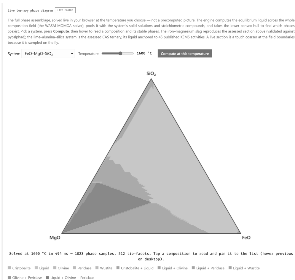
Figure 2: The live solver in the browser application (light theme). The user loads the shipped database, picks a temperature, and presses Compute; the WebAssembly engine then solves the full \text{FeO-MgO-SiO}_2 phase assemblage client side (here 1023 composition samples and 512 tie-facets in under half a second). Tapping a composition reads its stable phases and pins it to a comparison list; hovering previews on desktop.
