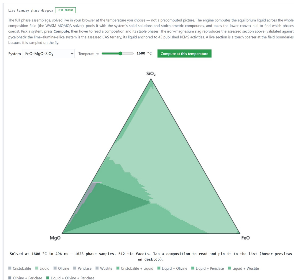
Figure 2: The live solver in the browser application (light theme). The user loads the shipped database, picks a temperature, and presses Compute; the WebAssembly engine then solves the full FeO-MgO-SiO 2 phase assemblage client side (here 1023 composition samples and 512 tie-facets in under half a second). Tapping a composition reads its stable phases and pins it to a comparison list; hovering previews on desktop.
