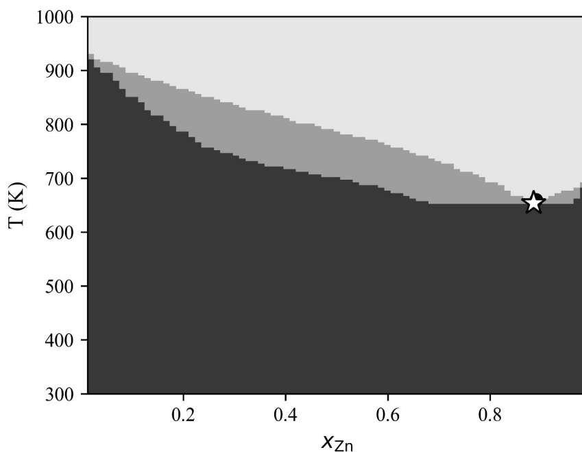
Figure 5: The Al-Zn phase diagram computed by the alloy listing from the shipped open TDB. Light to dark: liquid, liquid plus solid, and solid fields. The dot is the calculated eutectic (0.890, 660 K); the star is the assessed eutectic (0.885, 654 K).
