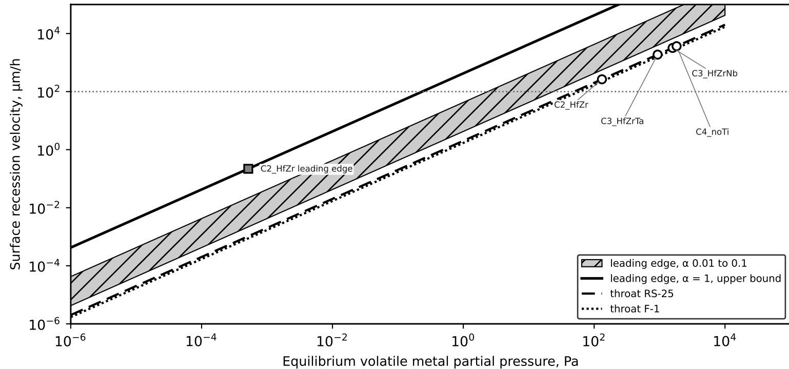
Recession From Measured Oxide Volatility, Four Survivors, RS-25 and F-1 Throats
