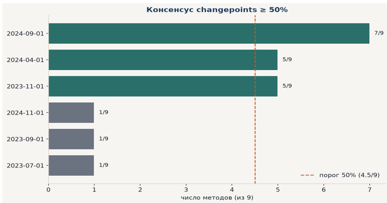
slide08_changepoint_consensus.png
