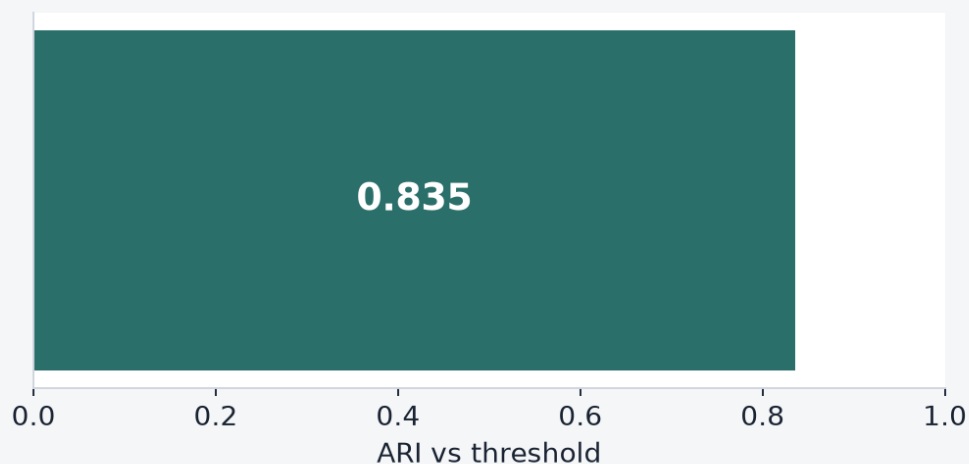
Louvain ARI \approx 0.835
