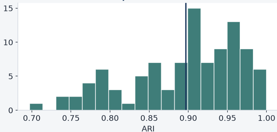
Bootstrap ARI 0.897 \pm 0.070
