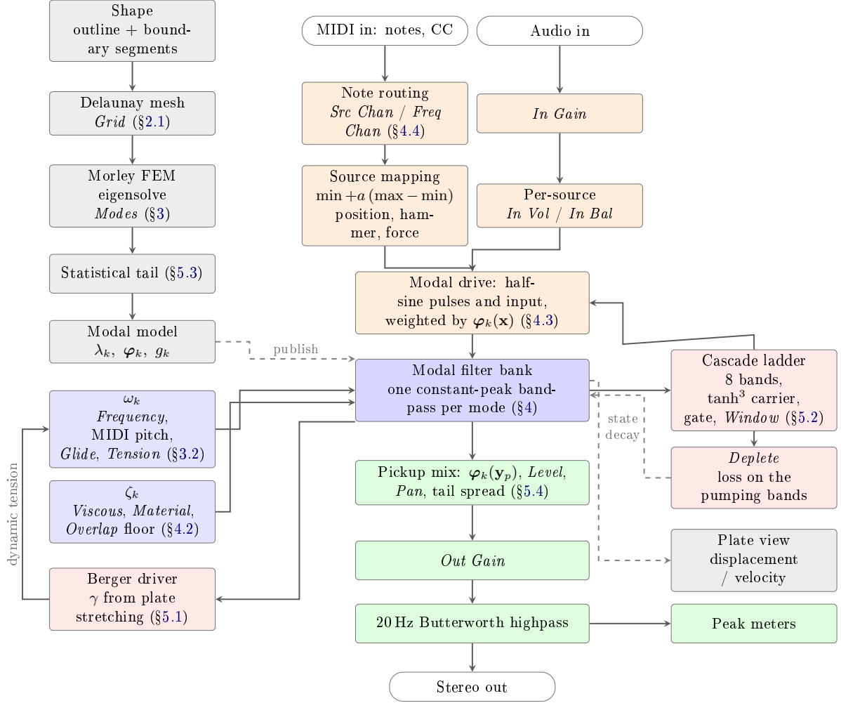
Figure 1: The complete signal path. Grey: the model, built on the message and background threads once per plate. Orange: excitation. Blue: the filter bank and what tunes it. Red: the two nonlinear feedback paths. Green: output. Dashed arrows carry state rather than signal. Everything but the grey column runs per sample on the audio thread. Italics name the control as it is labelled in the interface.
