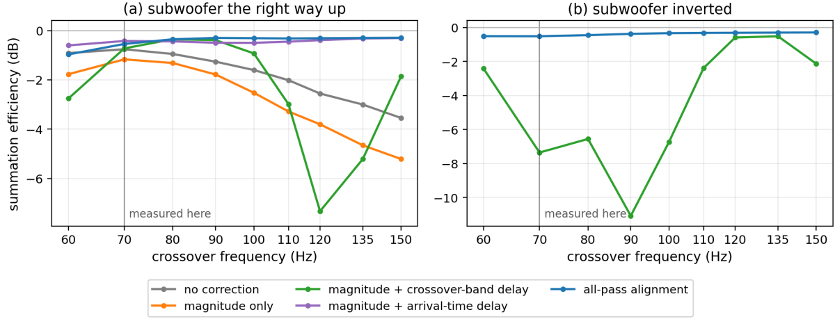
Figure 3: Summation efficiency against crossover frequency, averaged over both mains and all ten positions, with the subwoofer the right way up (a) and inverted (b). Only the crossover varies; the analysis range, the smoothing and the subwoofer routing level stay as the campaign set them. Every point is a prediction of (9) from the per-loudspeaker captures, not a measurement: the vertical line marks the one crossover that was measured, and the sweep starts at 60 Hz because below that the scored band [f_x/2, 2f_x] reaches under the analysis edge and it is that, rather than the crossover, that moves the curves.
