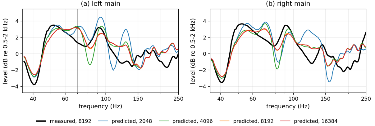
Figure 2: Filter length in the crossover region, for the two mains. Each curve is the linear-phase state averaged over the ten positions: the measured one, whose filter was rendered at 8192 taps, and the same design rendered at four lengths and put through (9). The 8192- and 16384-tap renderings lie on each other, to 0.03 dB RMS over the band drawn, and the measurement follows them to 1.2 dB. Shortening the filter parts company with them well before that: by 3.2 dB at 110 Hz on the left main at 2048 taps, and already by 2.0 dB and 2.3 dB near 81 Hz at 4096 — a feature of the length, not of the design.
