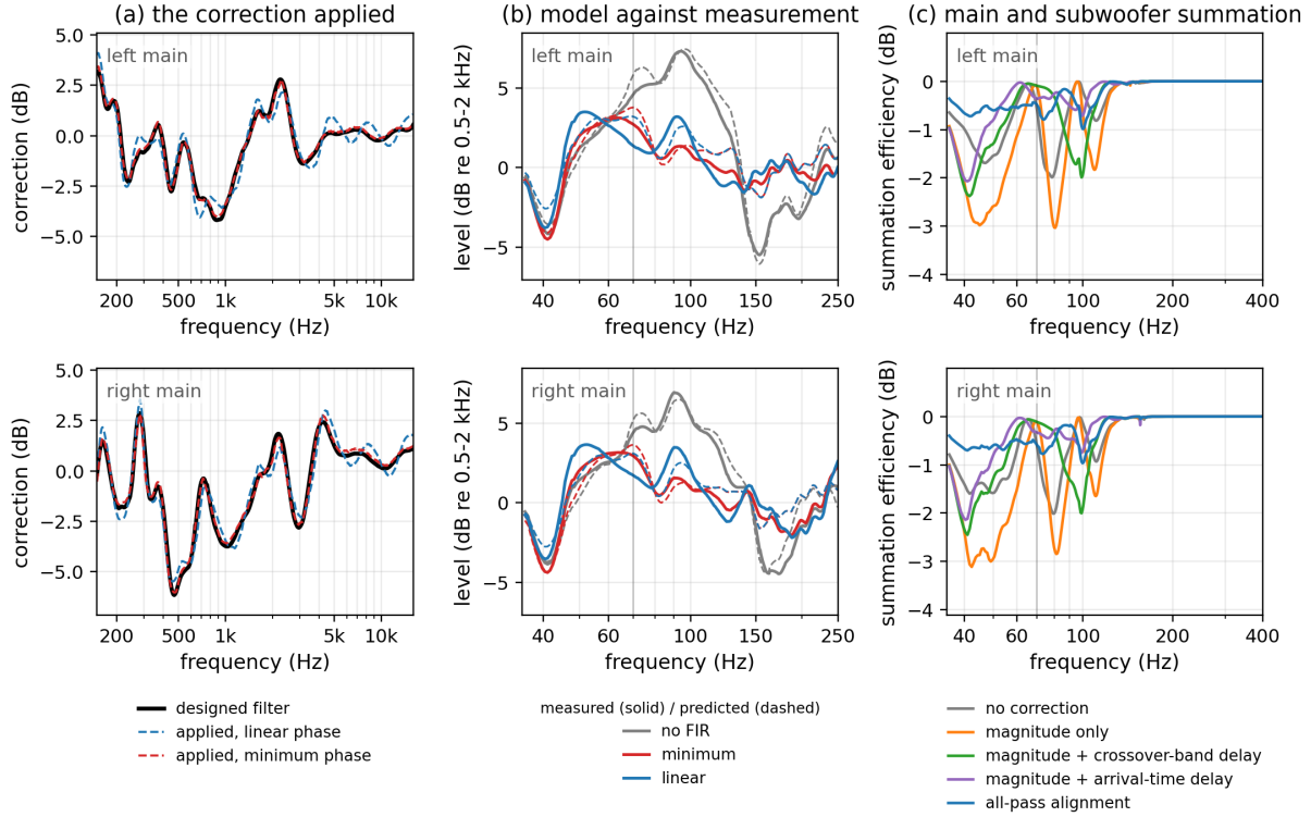
Figure 1: Both main loudspeakers with the subwoofer, the left on the top row and the right on the bottom; each column shares its vertical range between the two. (a) The correction the system applies, measured as the ratio of each corrected run to the uncorrected one at the same position, against the filter that was designed. (b) The three measured states through the crossover, averaged over the ten positions, against the prediction of (9), averaged over the ten positions. (c) Summation efficiency through the crossover for five strategies, averaged over the ten positions of the design set. Both delay estimators are drawn, since a magnitude-only correction is sensitive to which of the two it is given where the all-pass is not. Zero is coherent addition.
