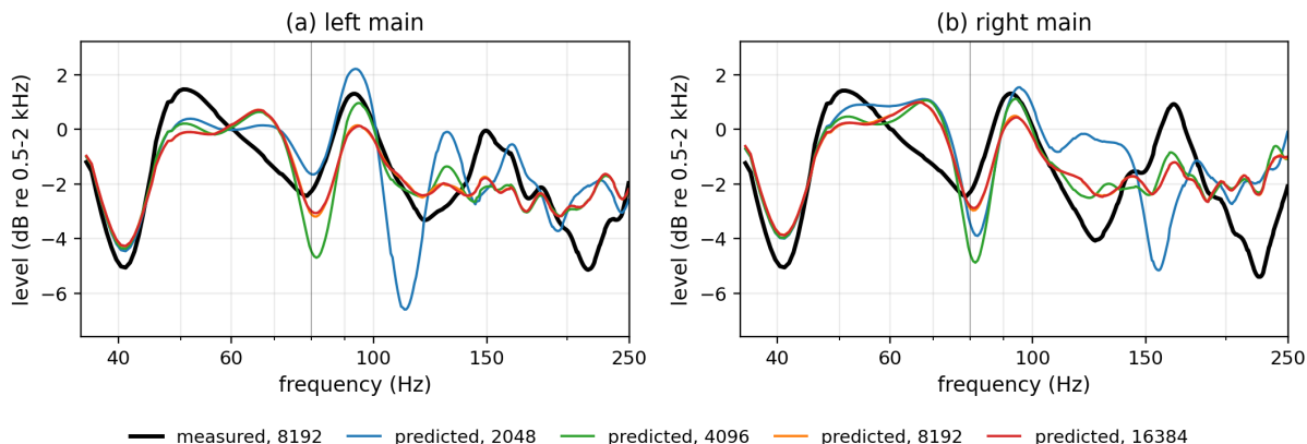
Figure 2: Filter length in the crossover region, for the two mains. Each curve is the linear-phase state averaged over the six shared positions: the measured one, whose filter was rendered at 8192 taps, and the same design rendered at four lengths and put through (9). The measurement follows the renderings from 8192 upwards, which lie on each other, and parts company with the 2048-tap one by 6 dB at 115 Hz on the left main — a feature of that length, not of the design.
