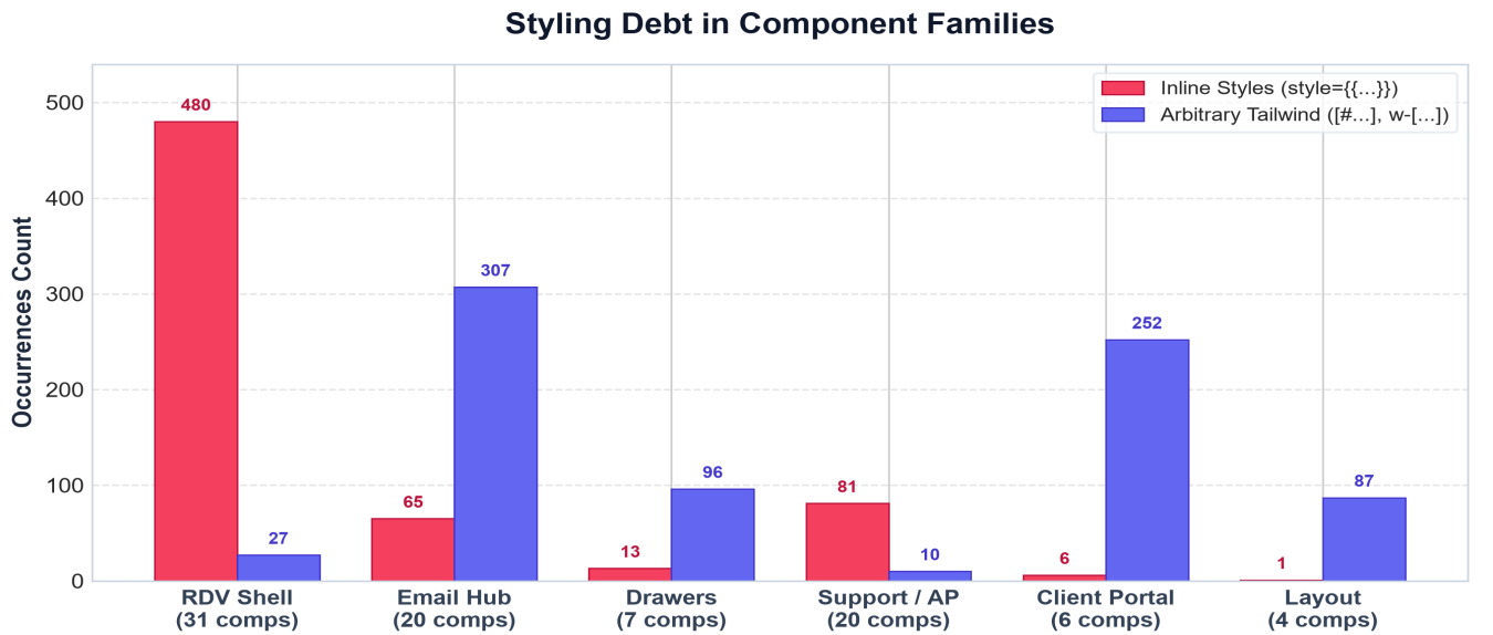
Figure 3: Raw Inline Styles vs. Arbitrary Tailwind Classes across Component Families.
