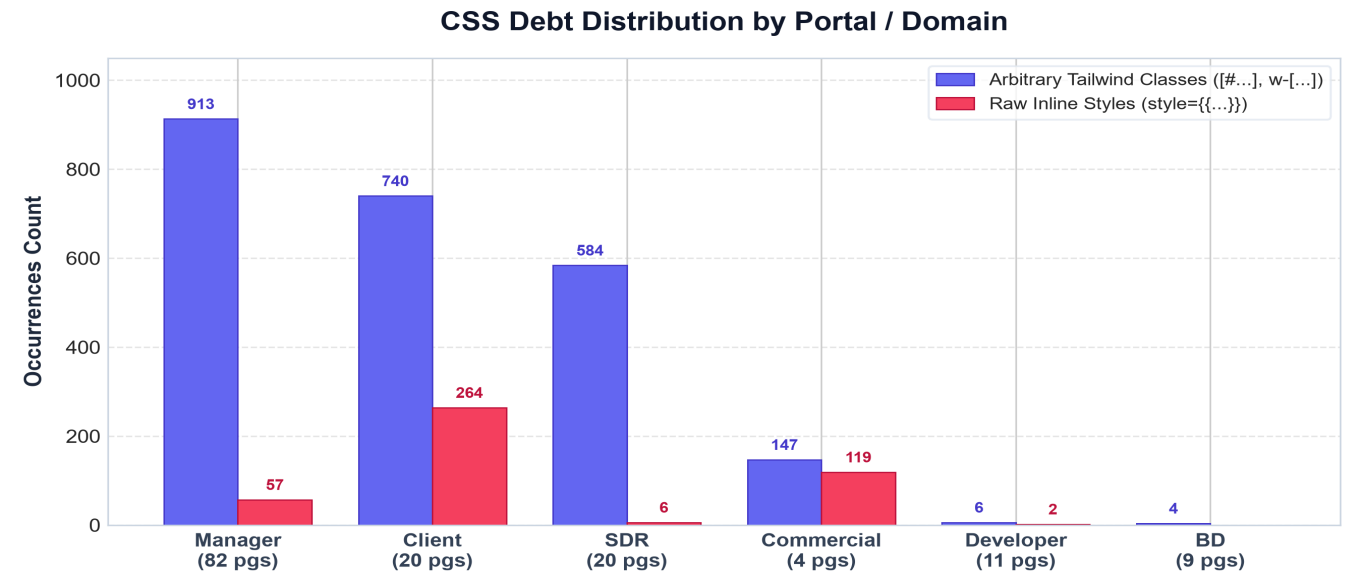
Figure 1: Distribution of Arbitrary Tailwind Bracket Classes vs. Raw Inline Styles across Application Portals.
