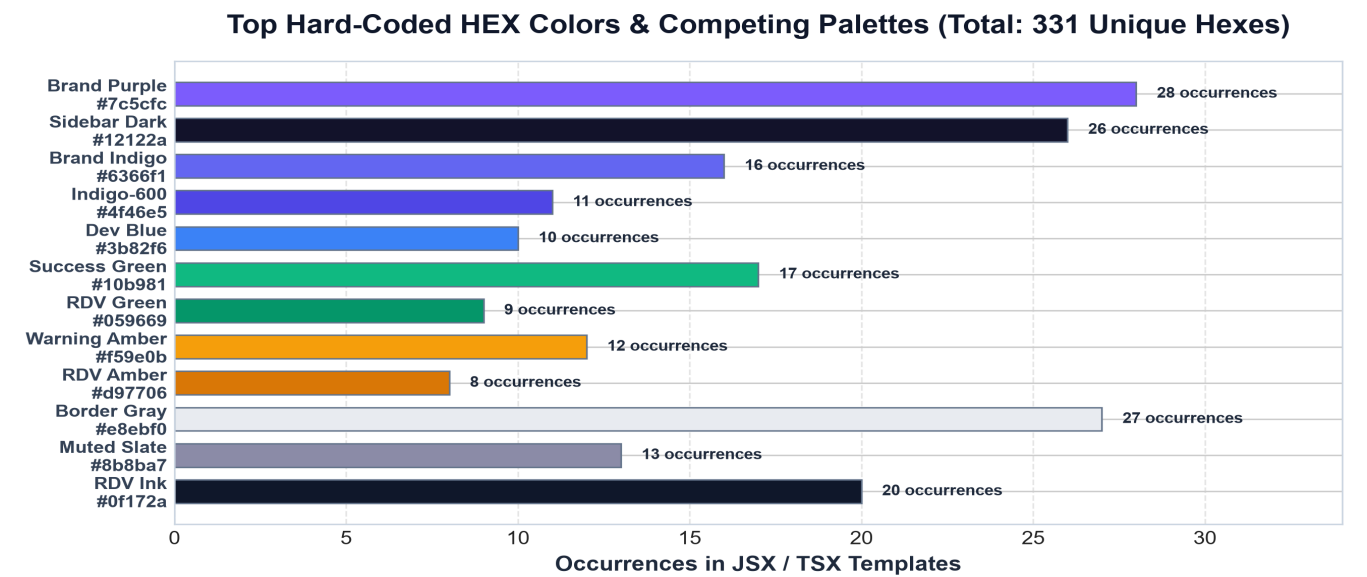
Figure 2: Top Hardcoded HEX Codes across TSX Templates & Their Competing Functional Roles.
