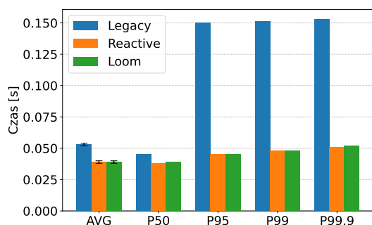
(c) wariant FIVE_SIMILAR
