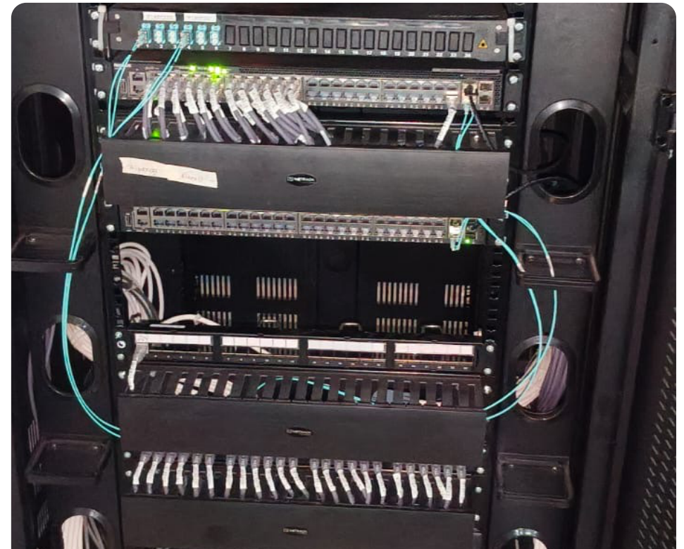
FIBER + ACCESS
