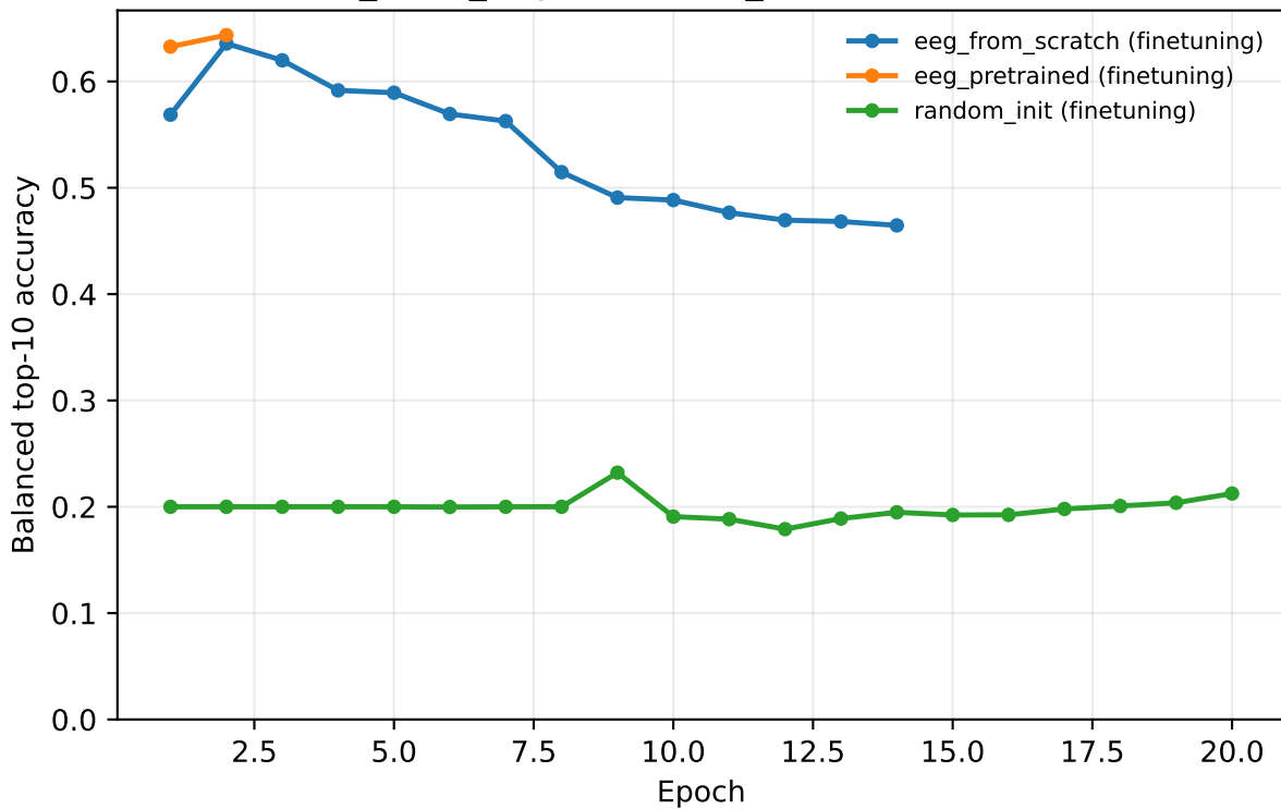
ds004408_three_way 20260702_144201 · val · retrieval 50
