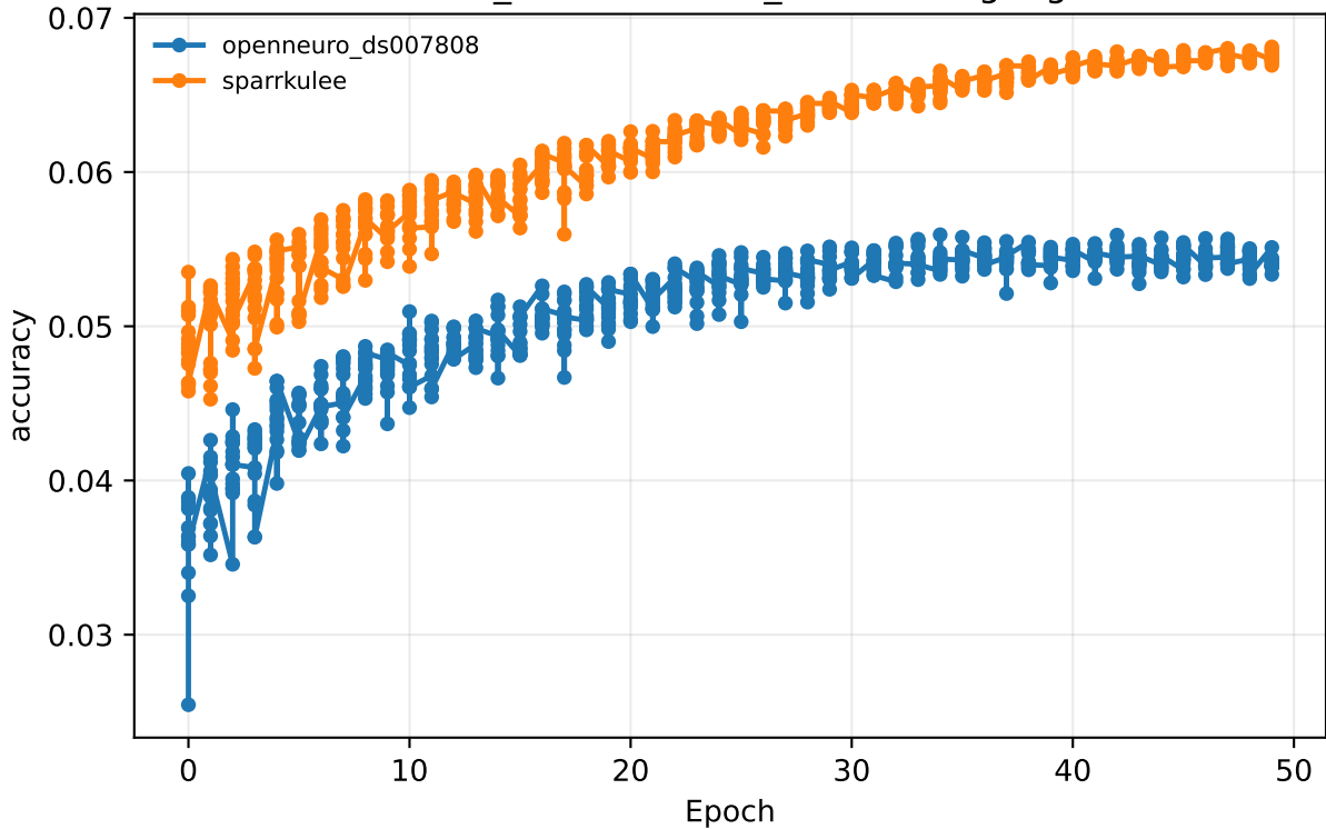
curriculum 20260629_004853 · from_scratch language · val/accuracy
