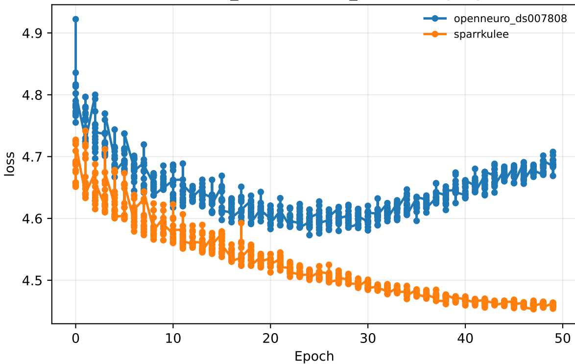
curriculum 20260629_004853 · from_scratch language · val/loss
