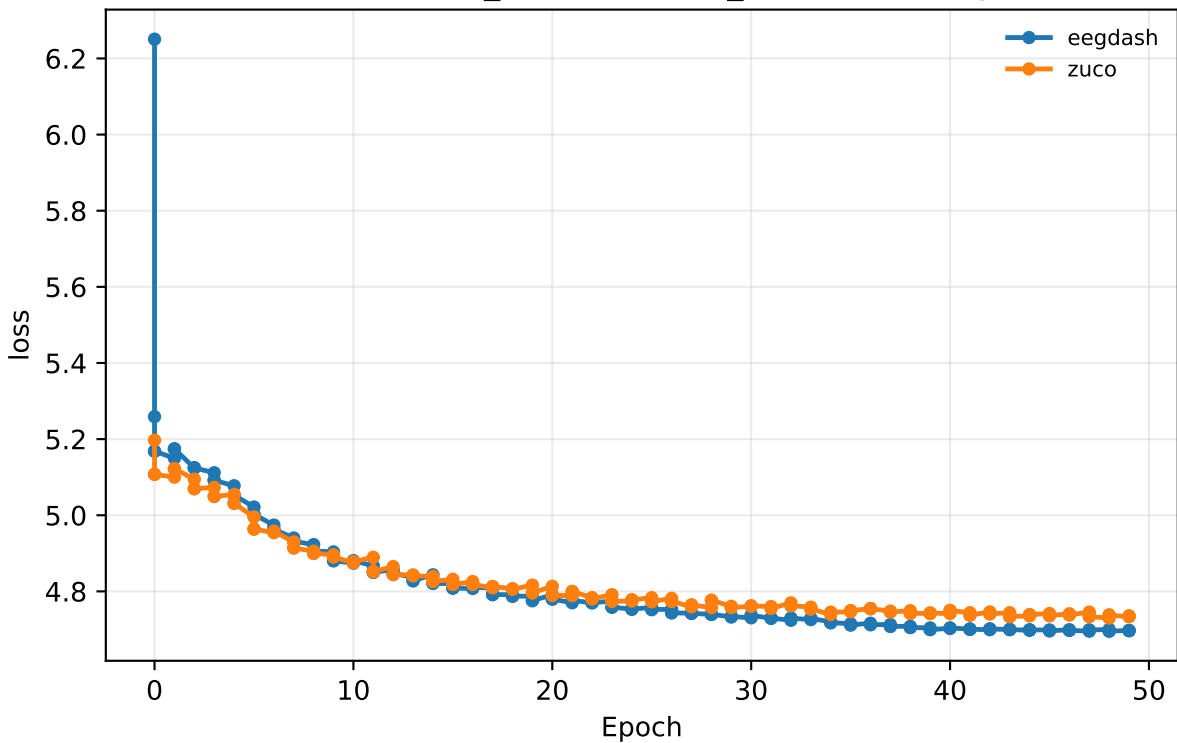
curriculum 20260629_004853 · from_scratch reading · val/loss
