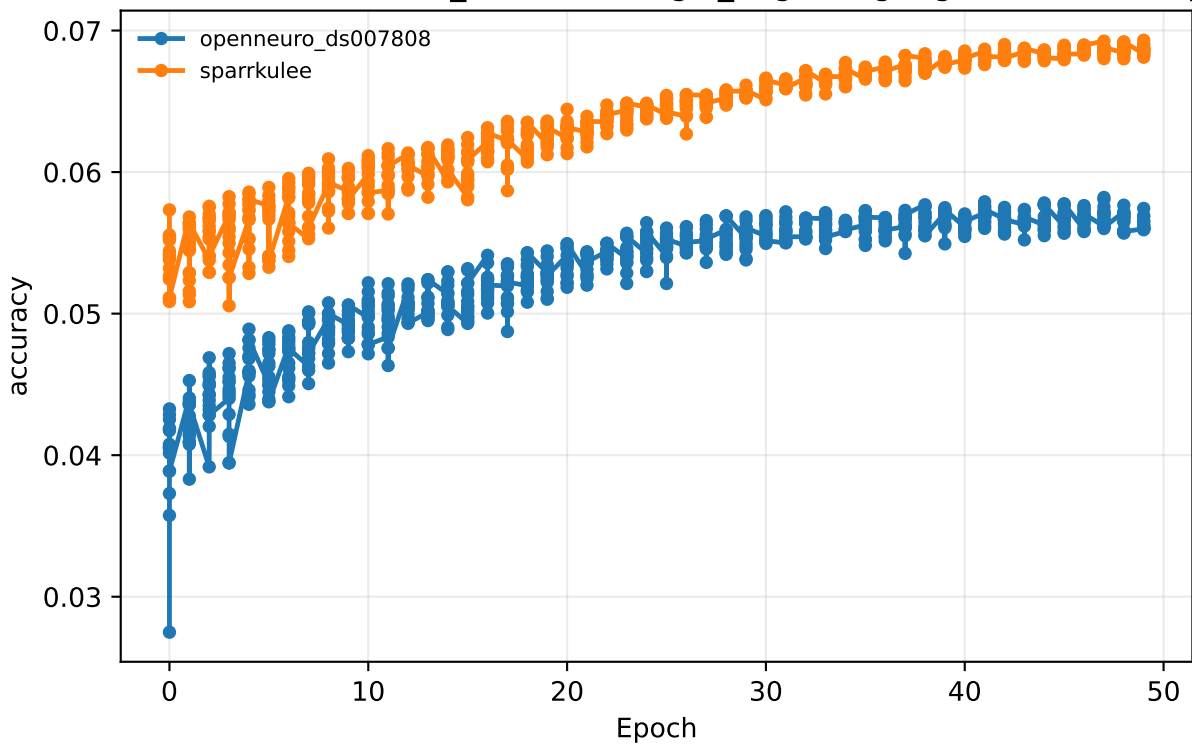
curriculum 20260629_004853 · megxl_eeg1 language · val/accuracy
