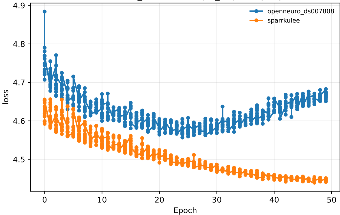
curriculum 20260629_004853 · megxl_eeg1 language · val/loss
