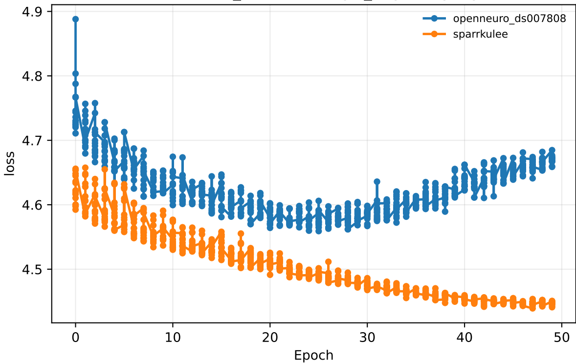
curriculum 20260629_004853 · megxl_eeg2 language · val/loss
