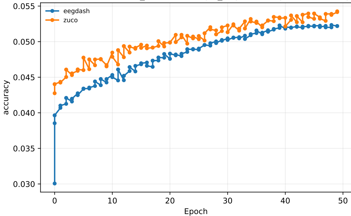
curriculum 20260629_004853 · megxl_eeg2 reading · val/accuracy
