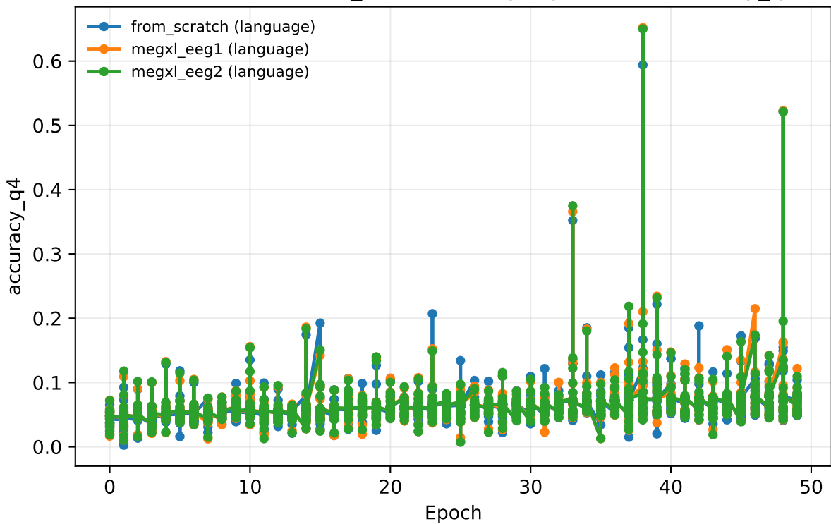
curriculum 20260629_004853 · language · train/accuracy_q4
