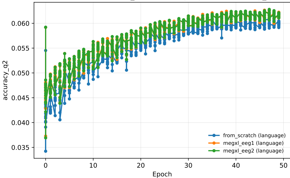
curriculum 20260629_004853 · language · val/accuracy_q2
