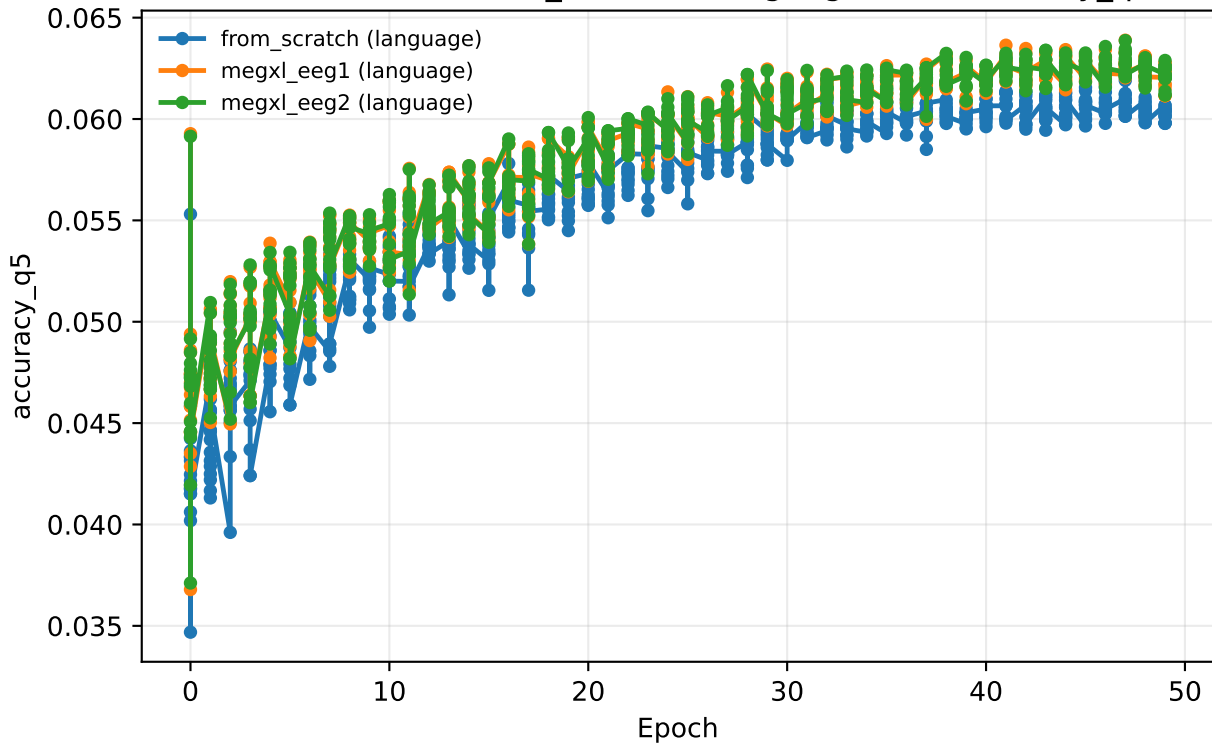
curriculum 20260629_004853 · language · val/accuracy_q5
