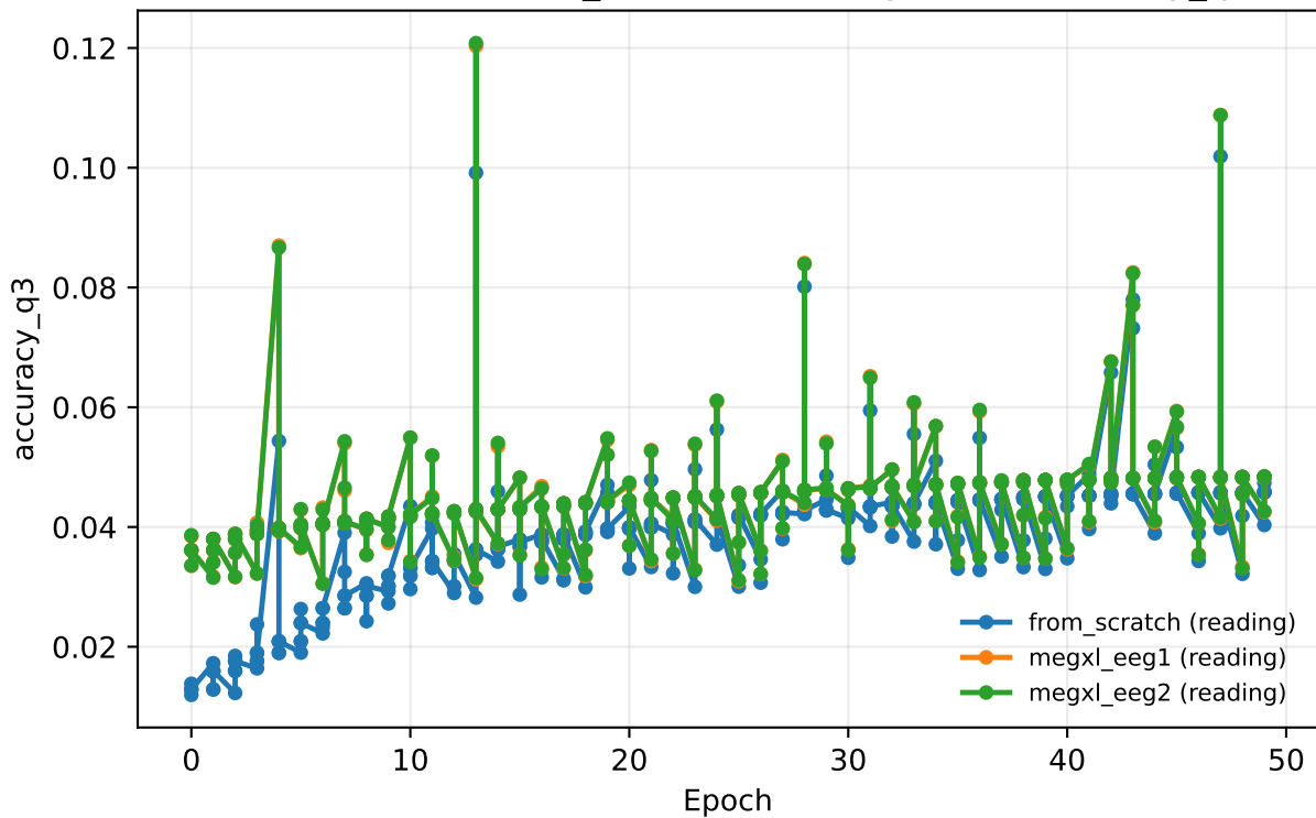
curriculum 20260629_004853 · reading · train/accuracy_q3
