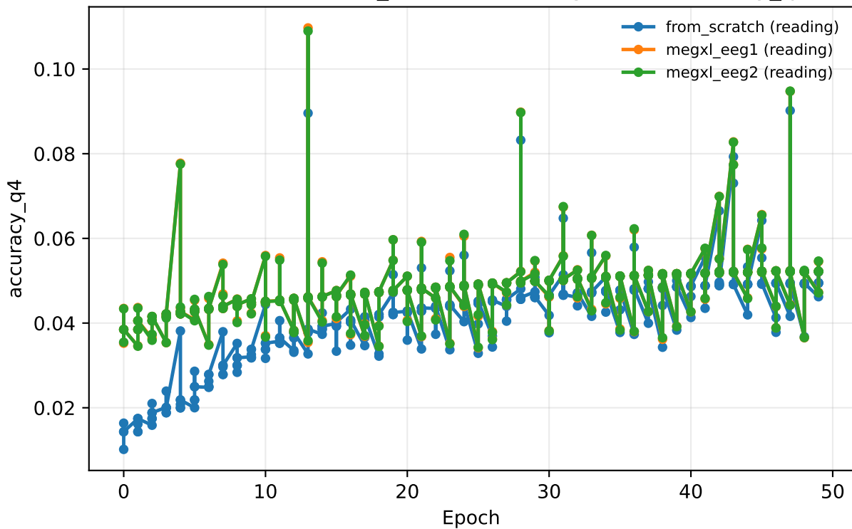
curriculum 20260629_004853 · reading · train/accuracy_q4
