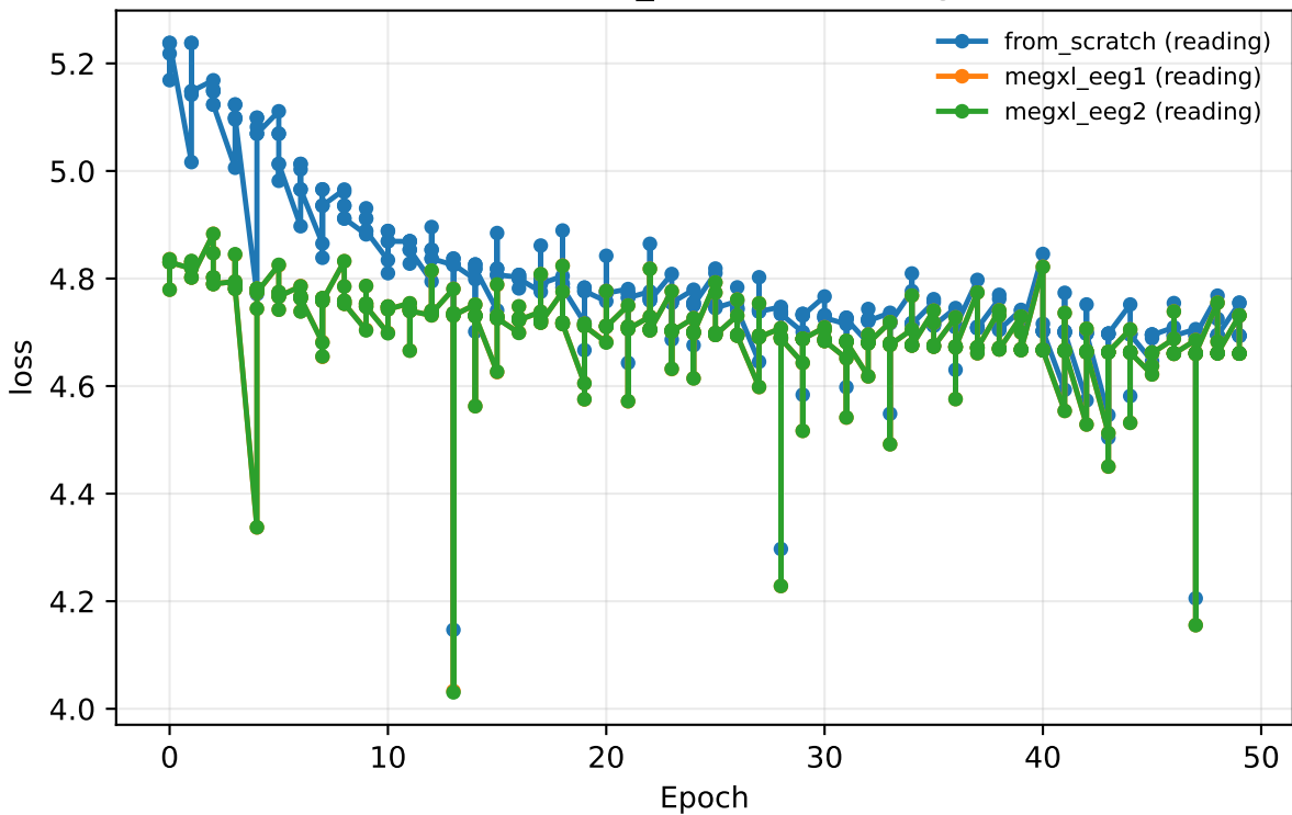
curriculum 20260629_004853 · reading · train/loss
