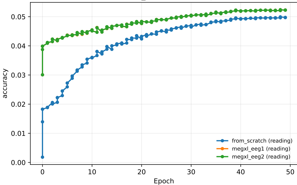
curriculum 20260629_004853 · reading · val/accuracy
