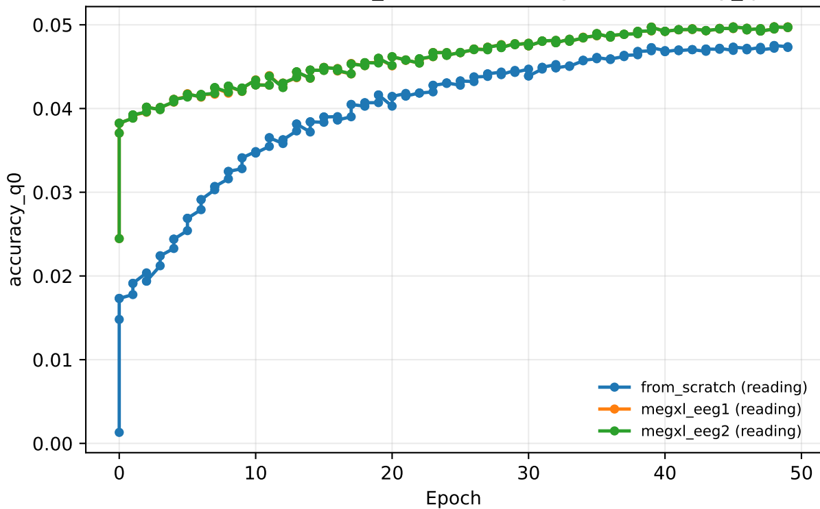
curriculum 20260629_004853 · reading · val/accuracy_q0
