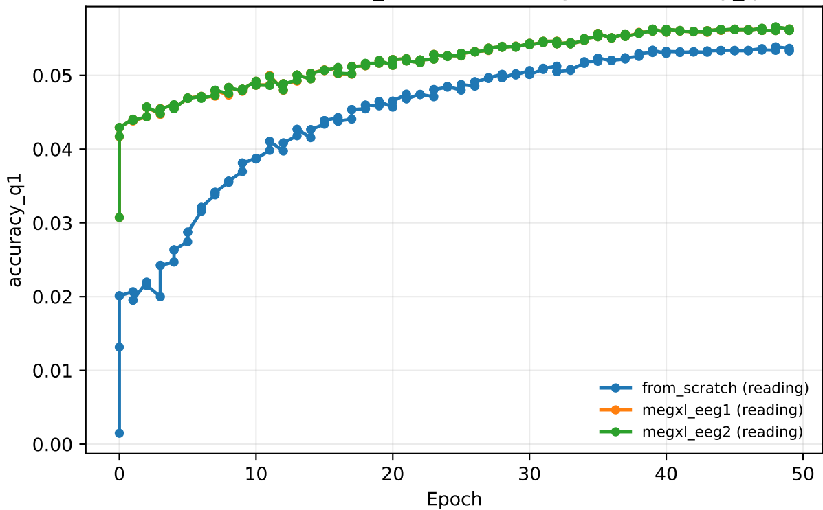
curriculum 20260629_004853 · reading · val/accuracy_q1
