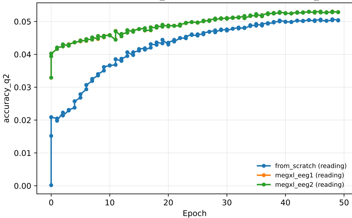
curriculum 20260629_004853 · reading · val/accuracy_q2
