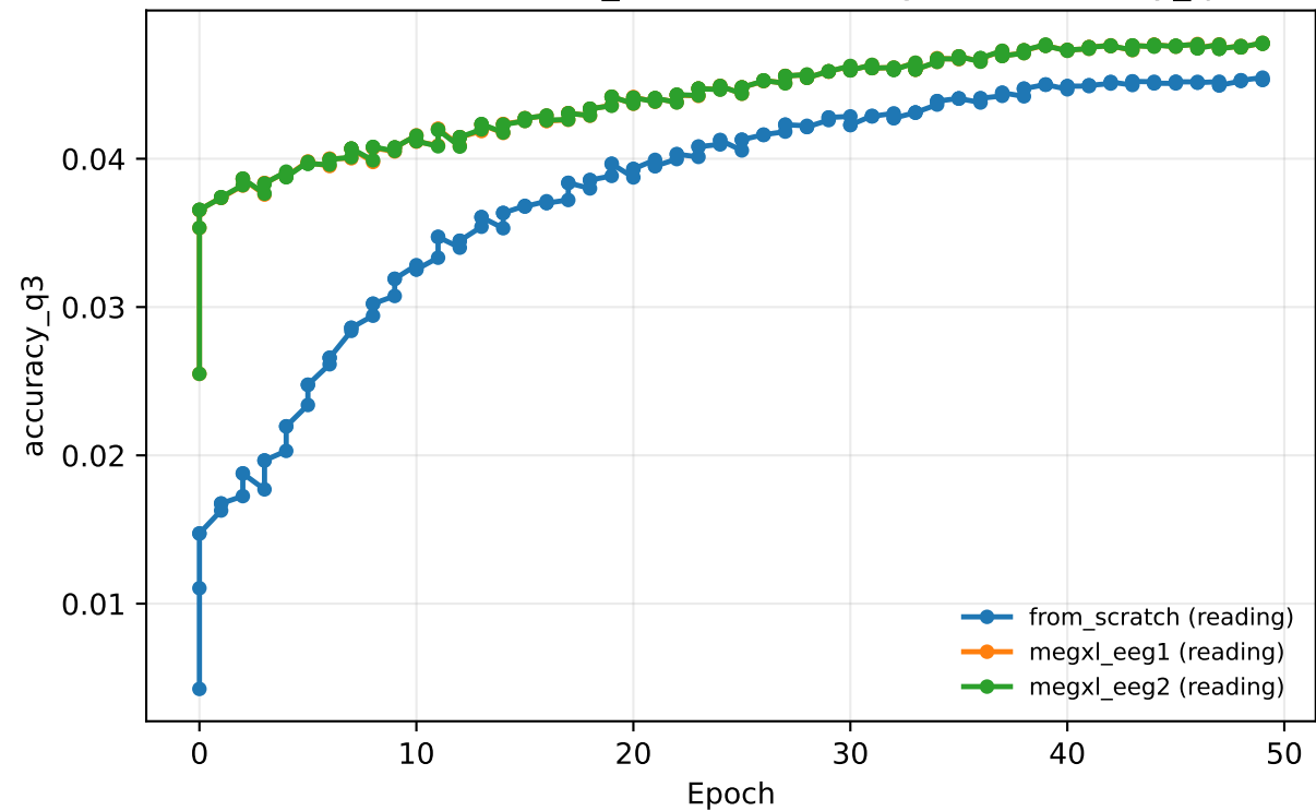
curriculum 20260629_004853 · reading · val/accuracy_q3
