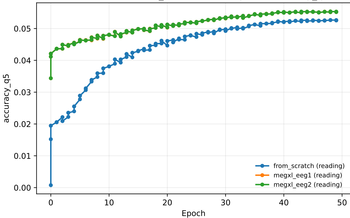
curriculum 20260629_004853 · reading · val/accuracy_q5
